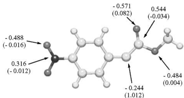
Fig. 6 Structure of \mathbf{3}^{\cdot-} calculated at the UB3LYP/6-31G(d) level of theory. Charge and spin densities (in parentheses) on the selected atoms are given in the structure drawing.
